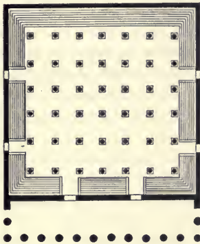
FIG. 35.—GROUND PLAN OF THE TELESTERION AT ELEUSIS
